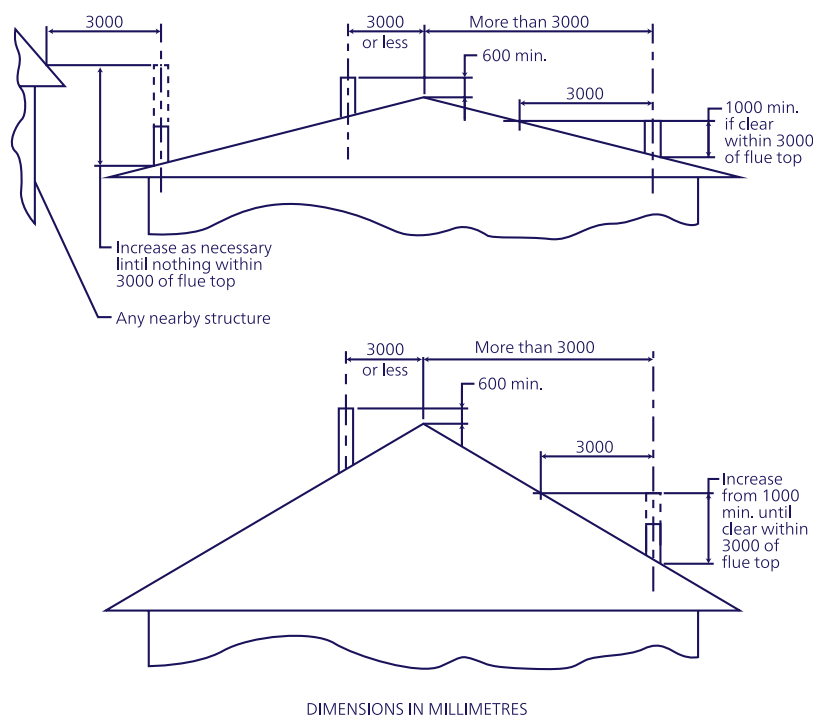
Figure 1. Minimum height of flue system
