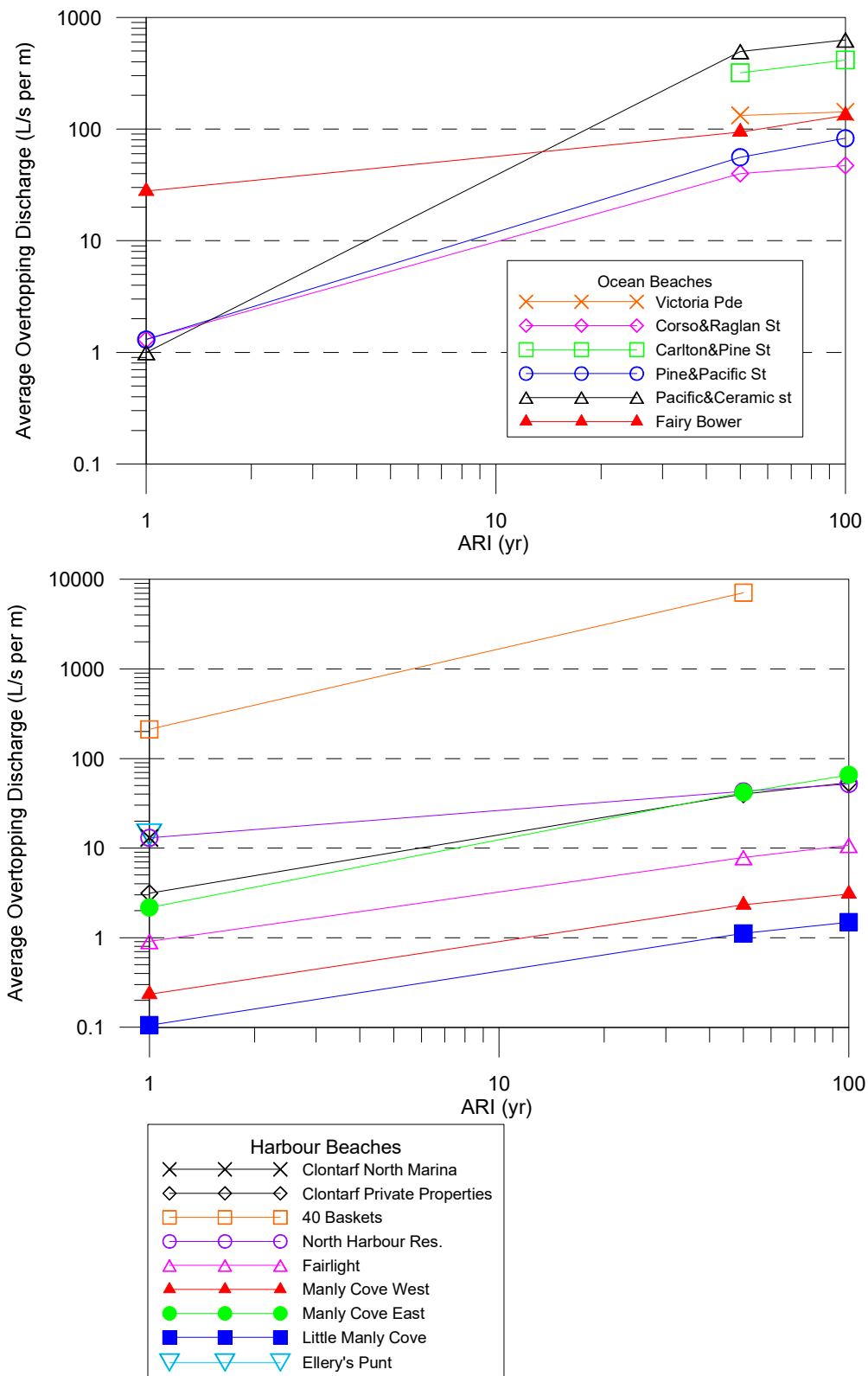
Figure 6.2 Plot of Present Day Predicted Overlapping Discharges
