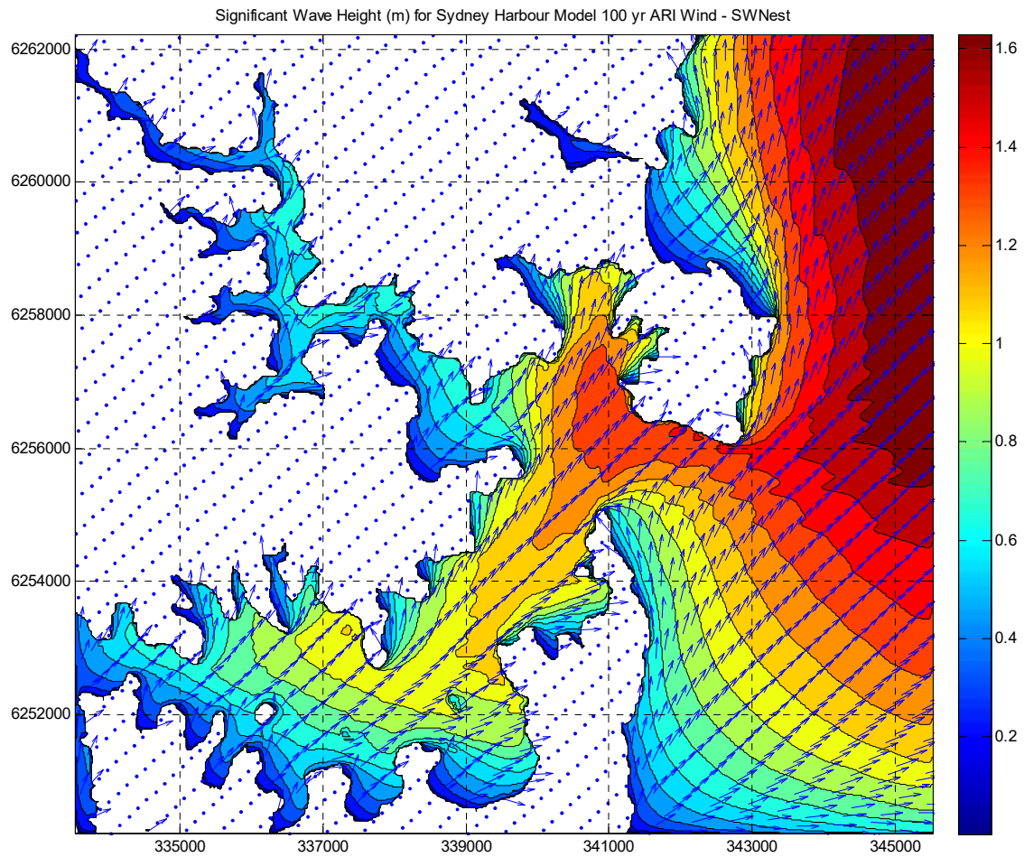
Figure 4.2 SWAN Model Results 100 Year ARI SW Wind Only
