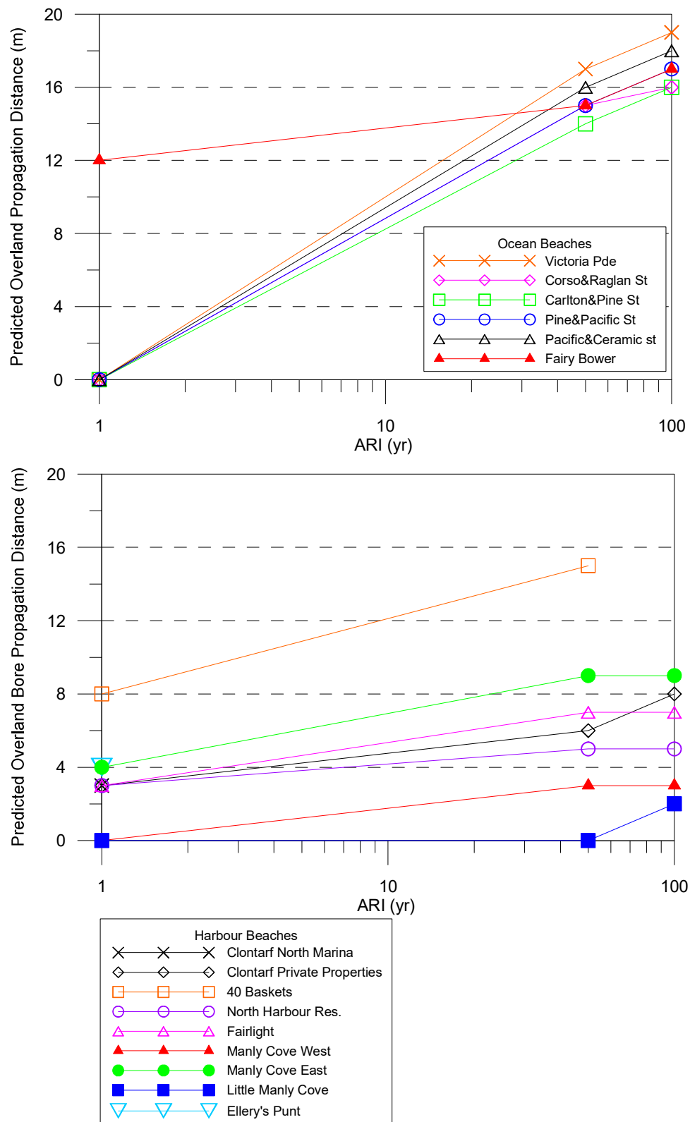
Figure 6.3 Plot of Present Day Overland Overtopping Propagation Distances
